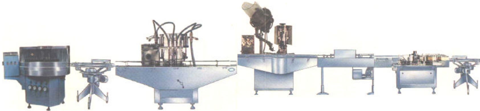
Typical Bottle Filling Line Station Points Program.
