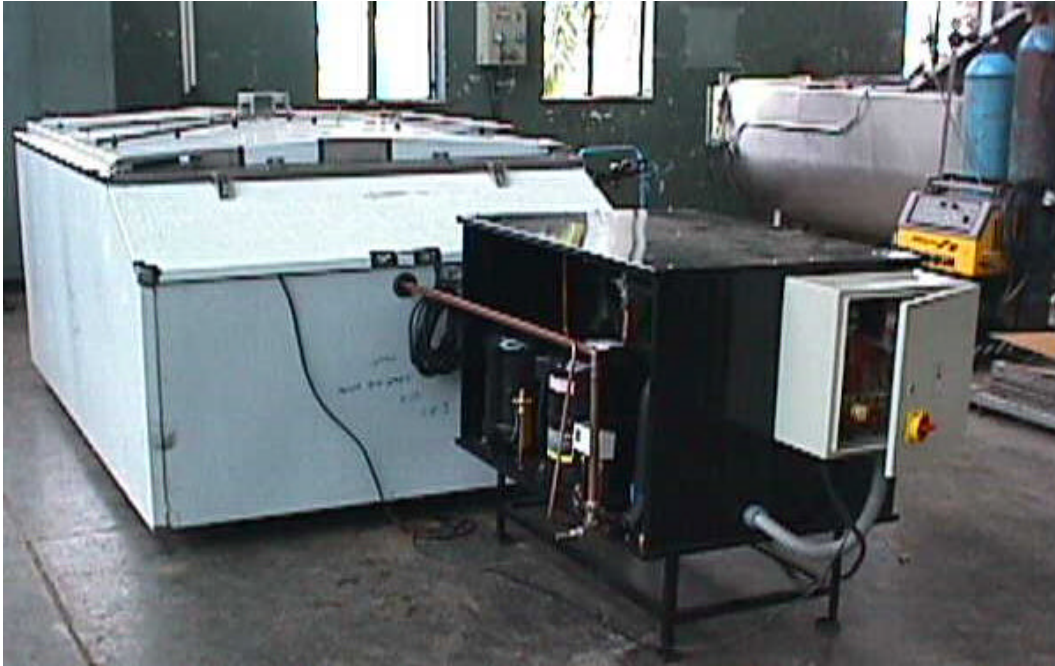
Actual Picture of 1,500 Litres Ice Bank Tank Type Milk Bulk Cooler Under Test on Factory Shop Floor.
